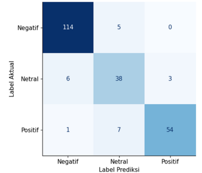
Confusion Matrix Model Terbaik — Linear SVM
